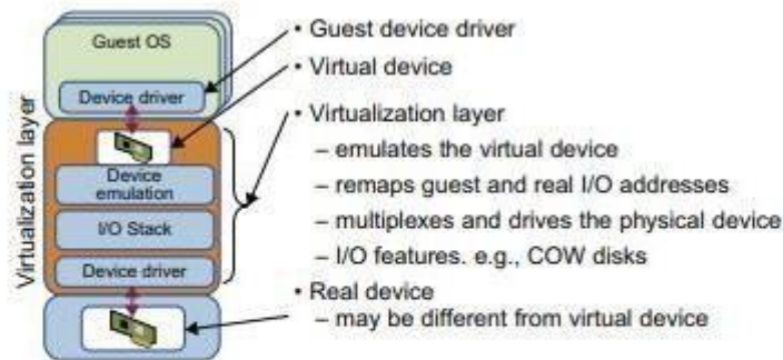
FIGURE 3.14 Device emulation for I/O virtualization implemented inside the middle layer that maps real I/O devices into virtual devices for the guest device driver to use.
